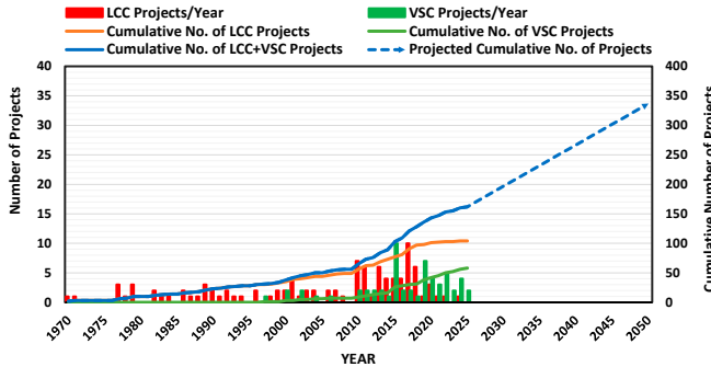
Figure 1 : DC Power Transmission Capacity since 1970
